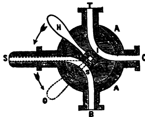
FIG. 14.—Papin's Two-Way Cock.
